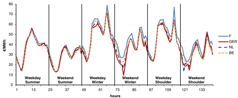
Fig. 3 Hourly nodal reference prices
