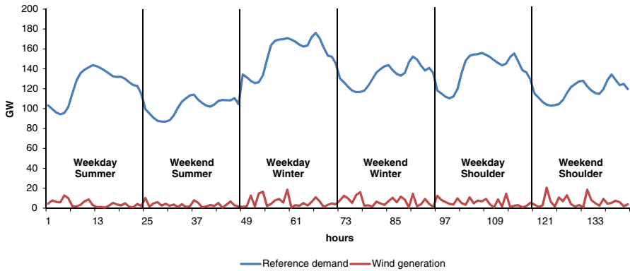
Fig. 4 Wind generation and overall reference demand
