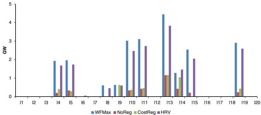
Fig. 5 Line extension results (final period)
