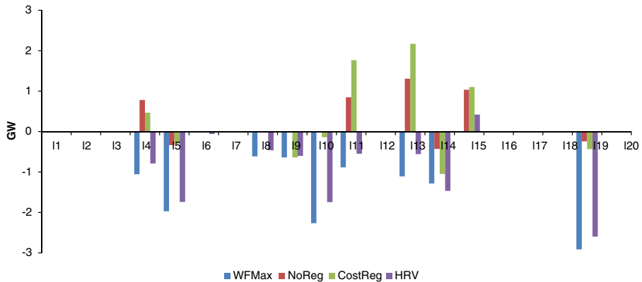
Fig. 12 Line extension differences between the simplified model and the baseline (final period)
