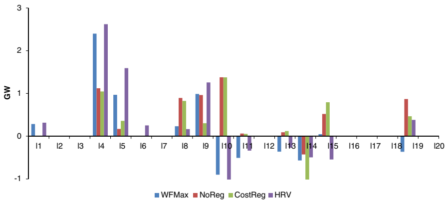
Fig. 10 Line extension differences between baseline and the case with increased wind capacity (final period)
