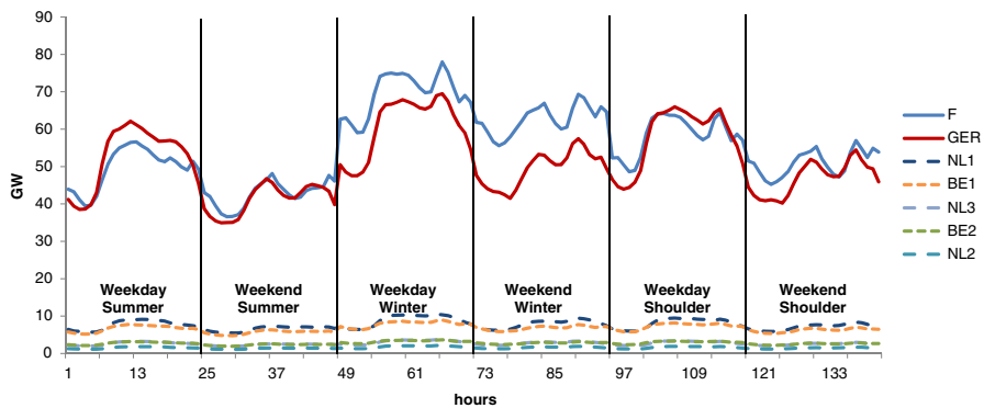
Fig. 2 Hourly nodal reference demand
