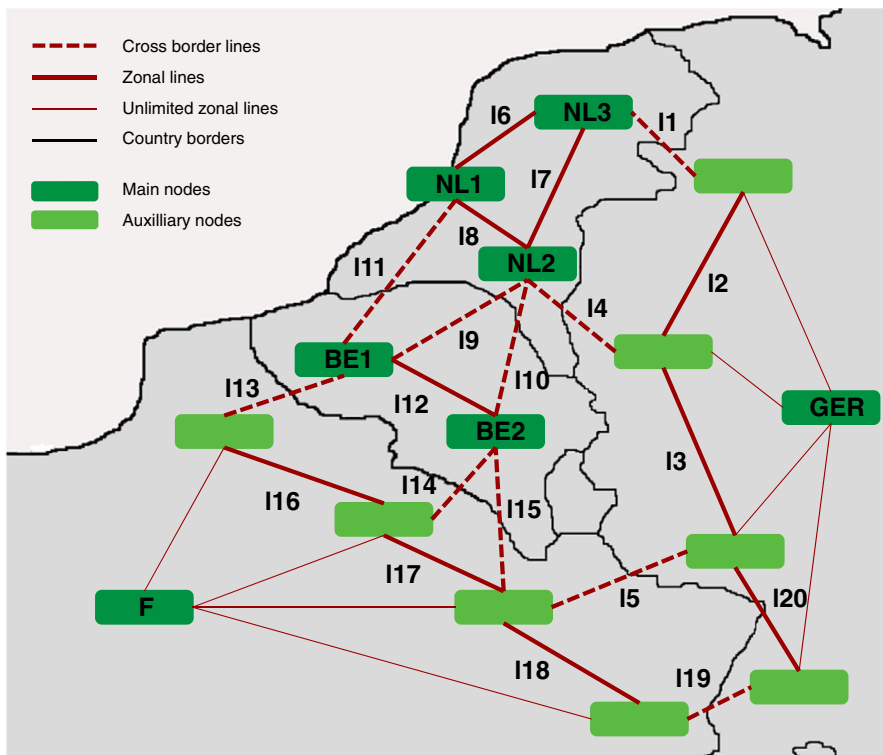
Fig. 1 The stylized Western European transmission network
