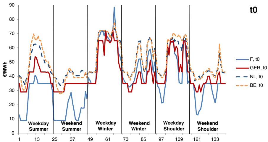
Fig. 7 Hourly nodal prices before network extension
