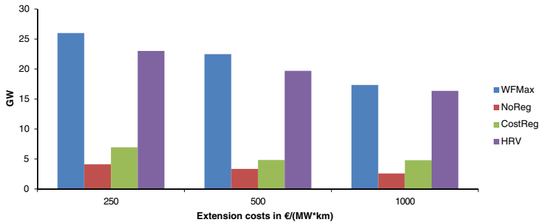
Fig. 9 Overall network extension for different cost assumptions
